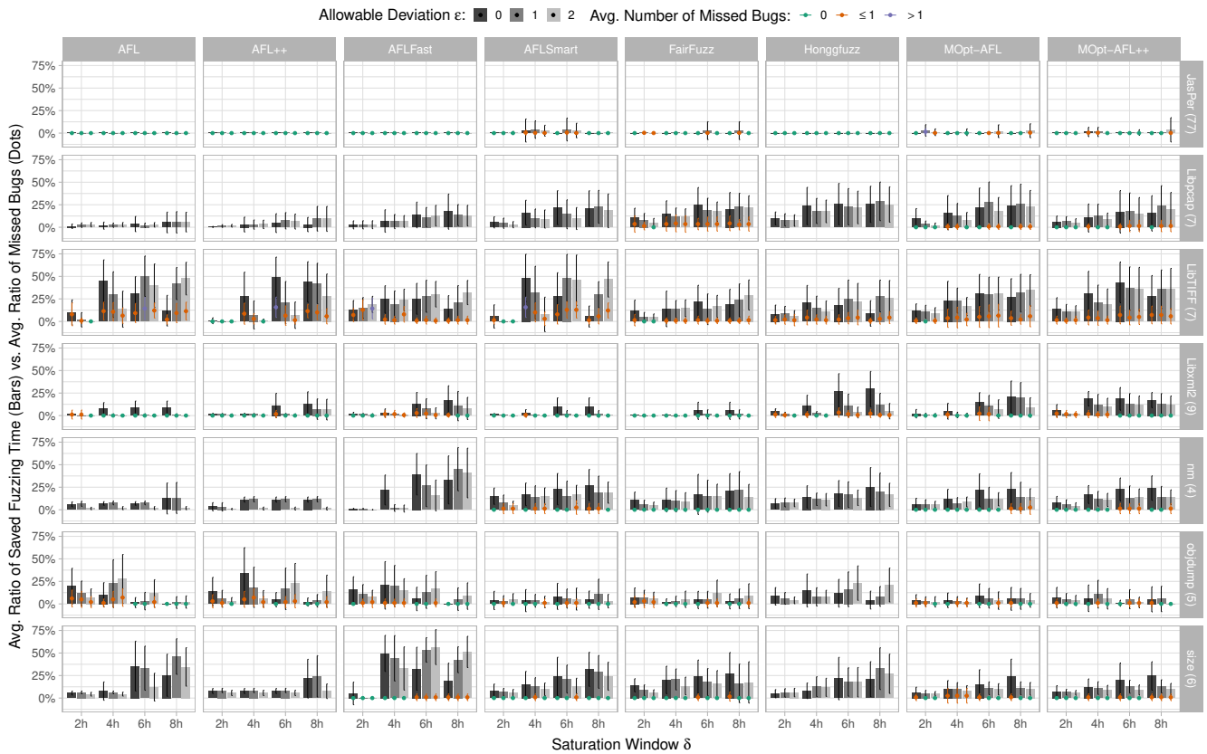
Figure 7: Tradeoff results of our stopping criterion relative to the saturation of regular function coverage.
